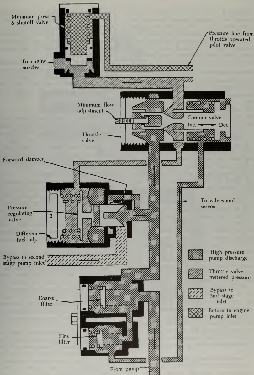
FIGURE 3-48. Metering system.
